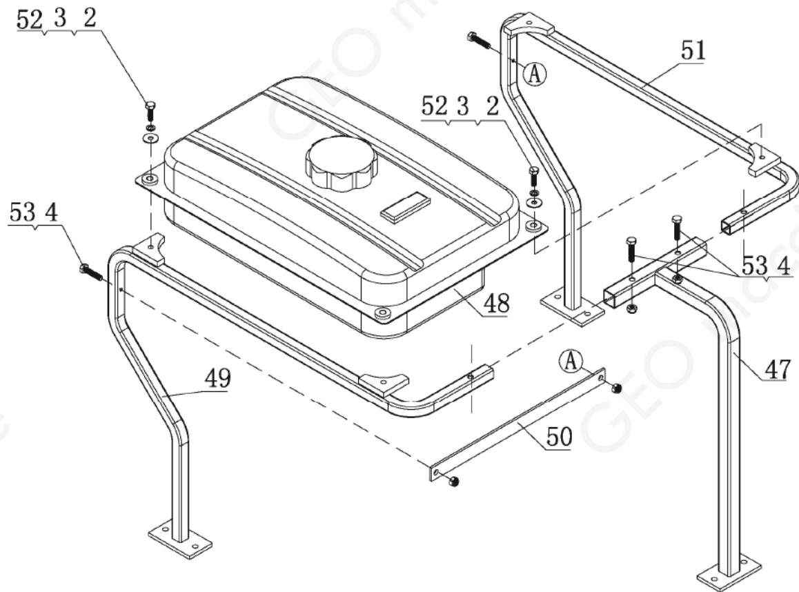
LM120_FuelTank
