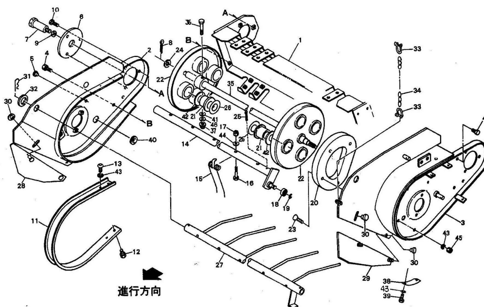
YK0850.YK0870 Round baler picking-up assy
