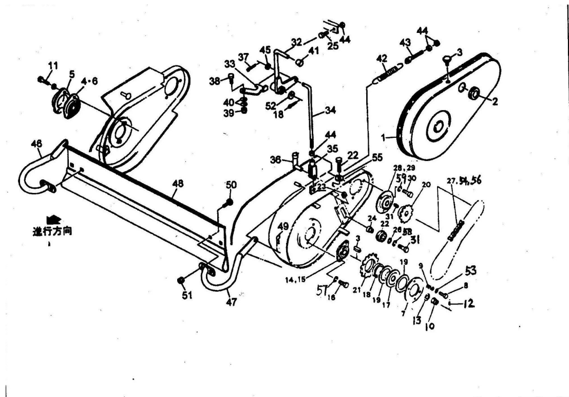
YK0850. YK0870 Round baler Picking-up sprocket Assy
